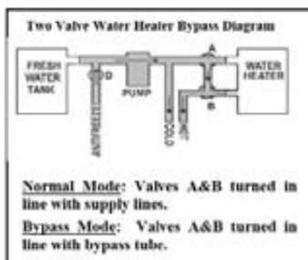
Two Valve Water Heater Bypass
